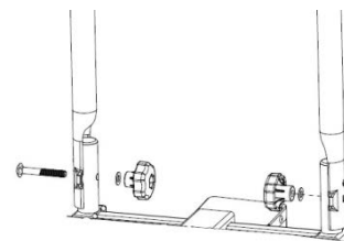
Figure 2: Assembly of U-shaped bracket
